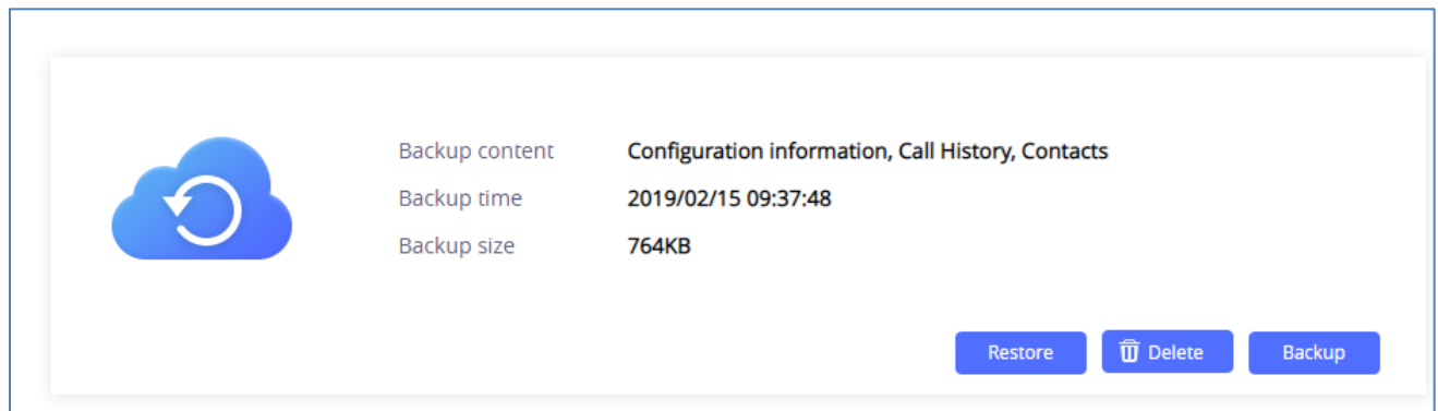
Figure 53: Generated Backup
